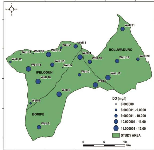
Fig.4 Risk map showing DO concentration in the study area
