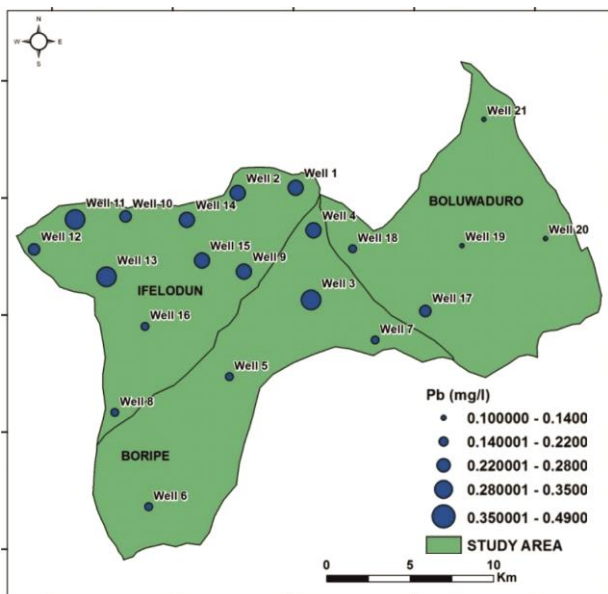
Fig3 Risk map showing Pb concentration in the study area
